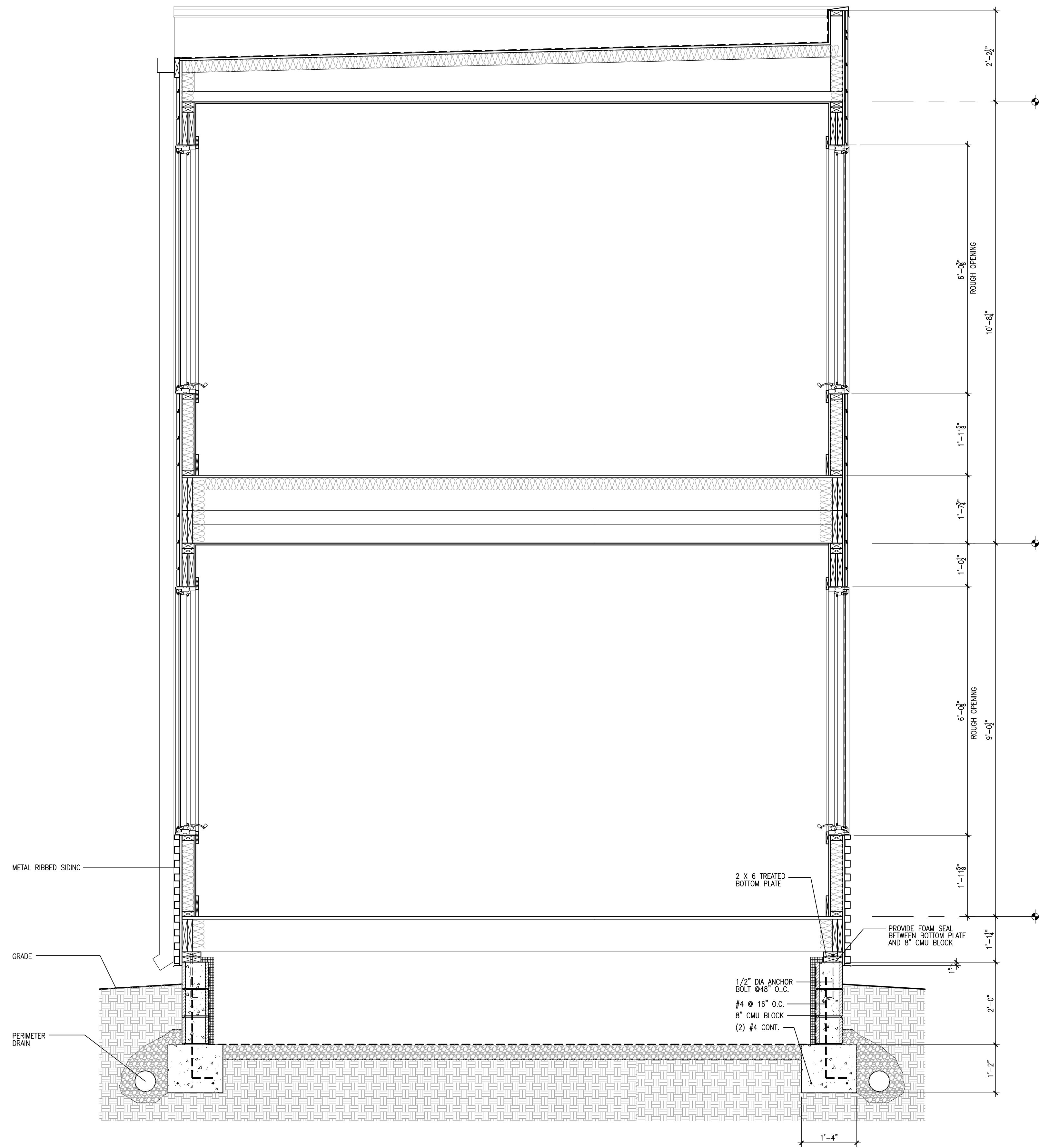
② BUILDING SECTION SCALE: 3/4"=1'-0"
