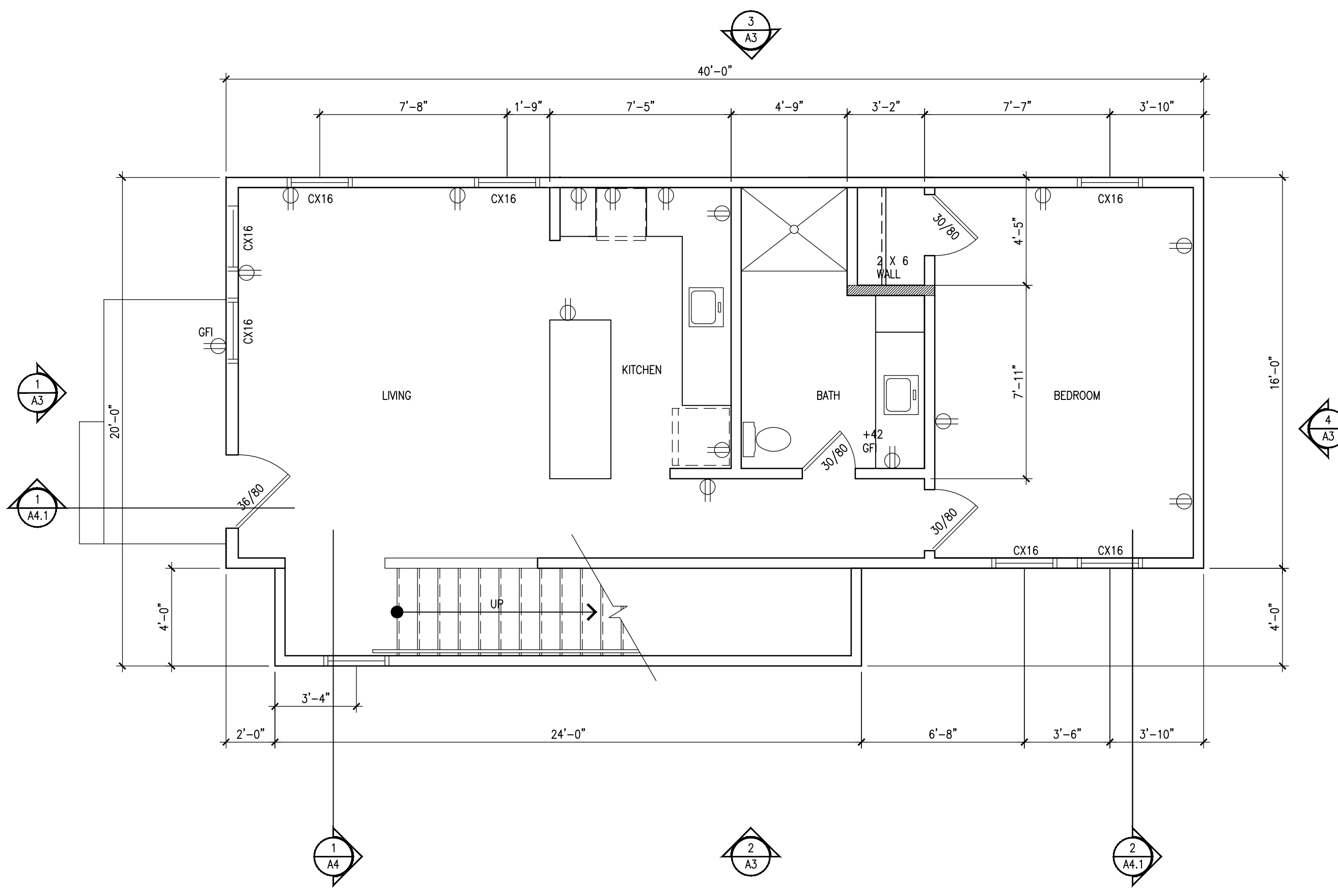
1 FIRST FLOOR SCALE: 1/4"=1'-0"
