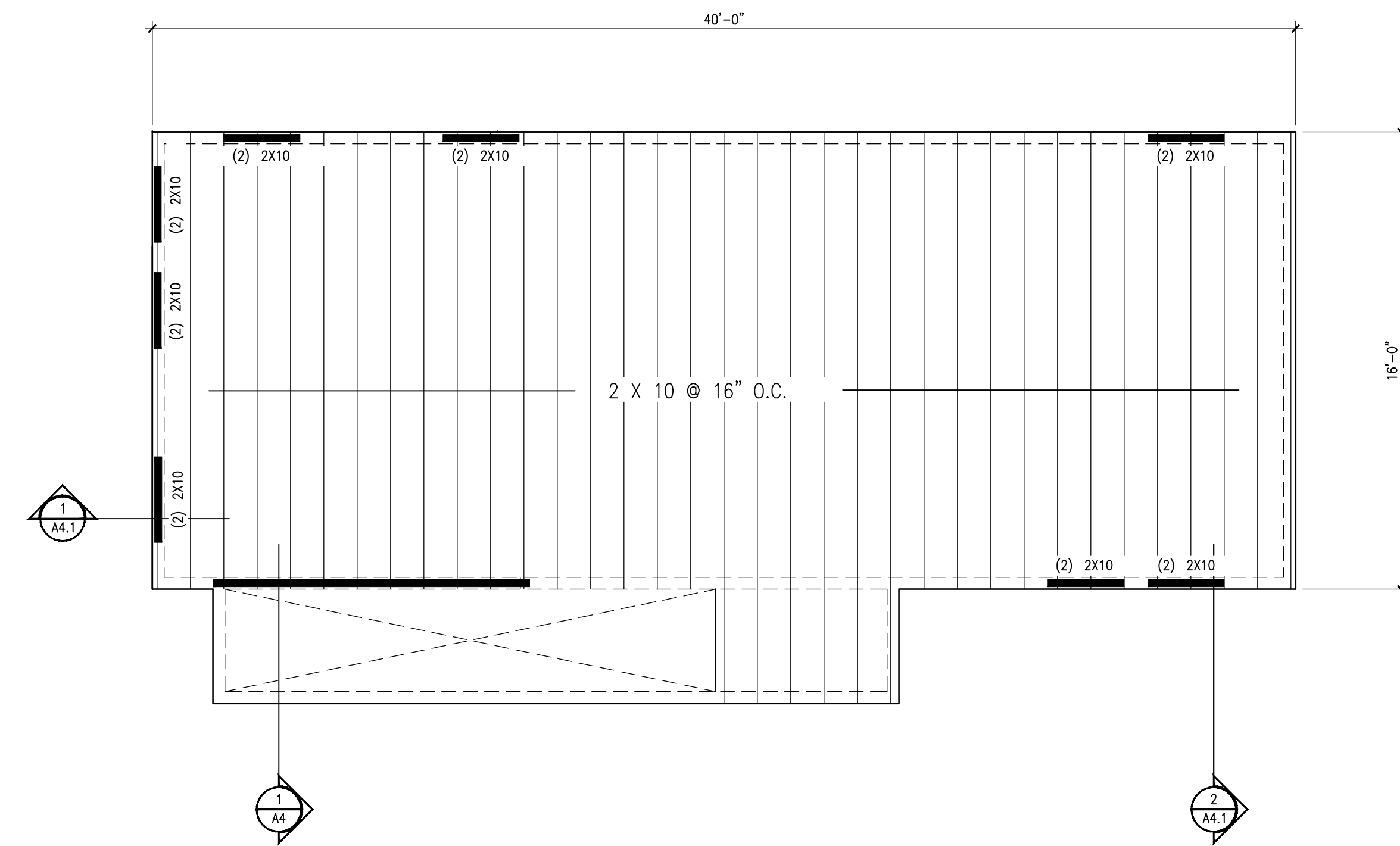
3 SECOND FLOOR FRAMING PLAN SCALE: 1/4"=1'-0"
