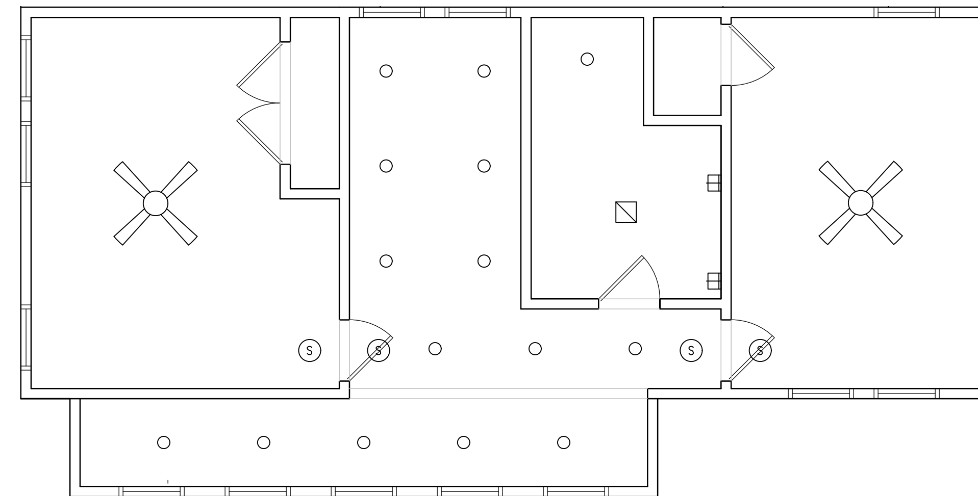
② SECOND FLOOR CEILING PLAN SCALE: 1/4"=1'-0"
