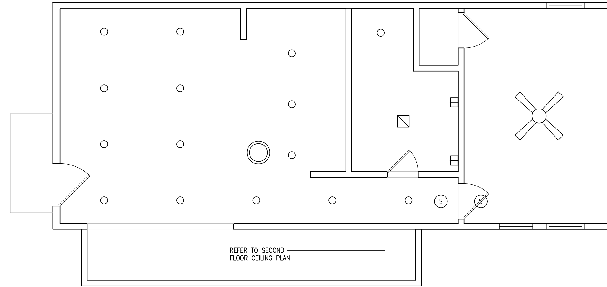
① FIRST FLOOR CEILING PLAN SCALE: 1/4"=1'-0"
