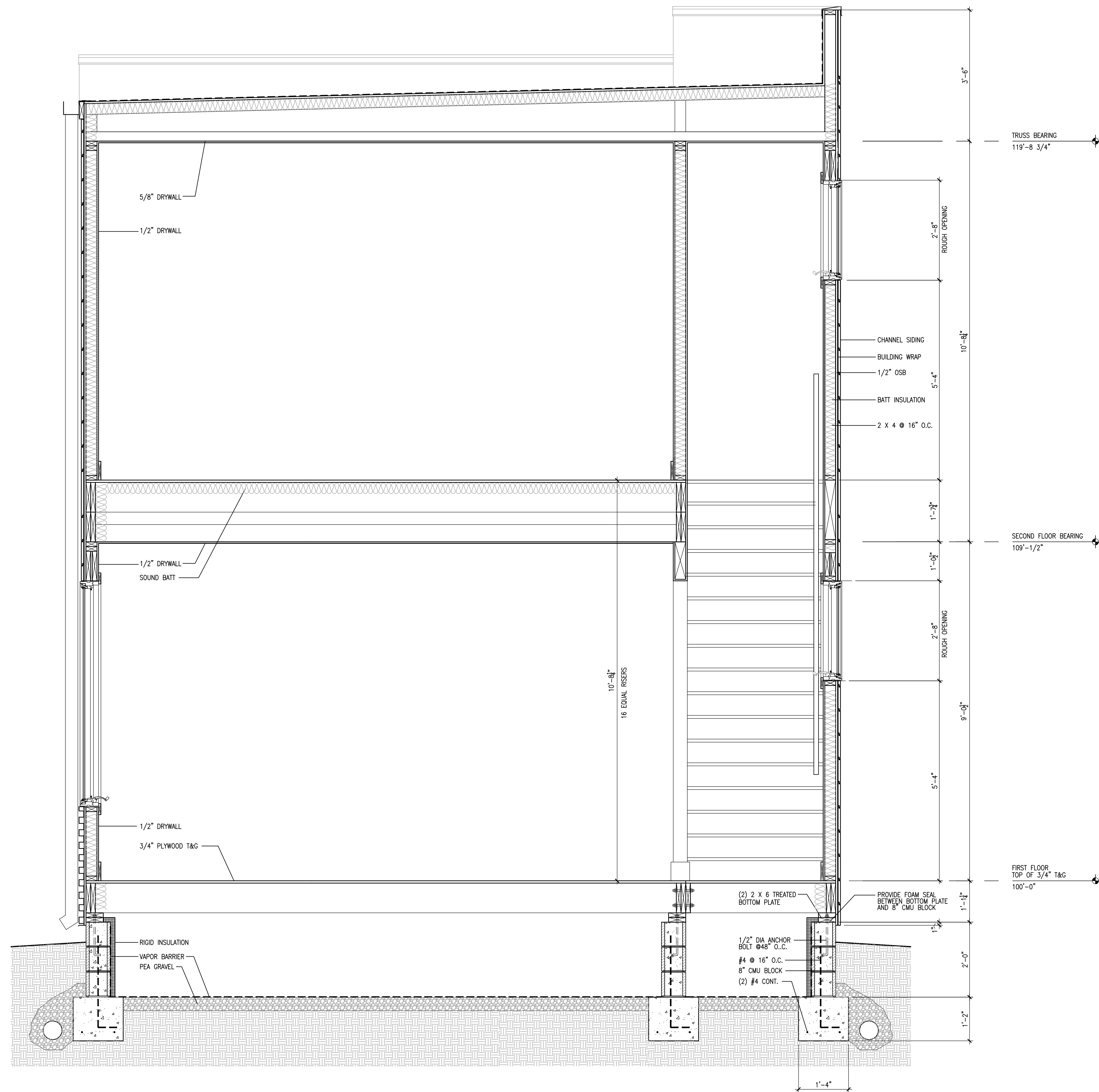
1 BUILDING SECTION SCALE: 3/4"=1'-0"
