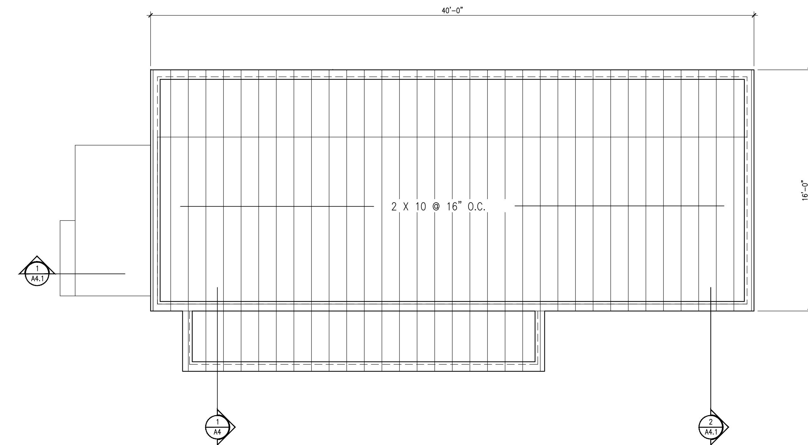
2 FIRST FLOOR FRAMING PLAN SCALE: 1/4"=1'-0"
