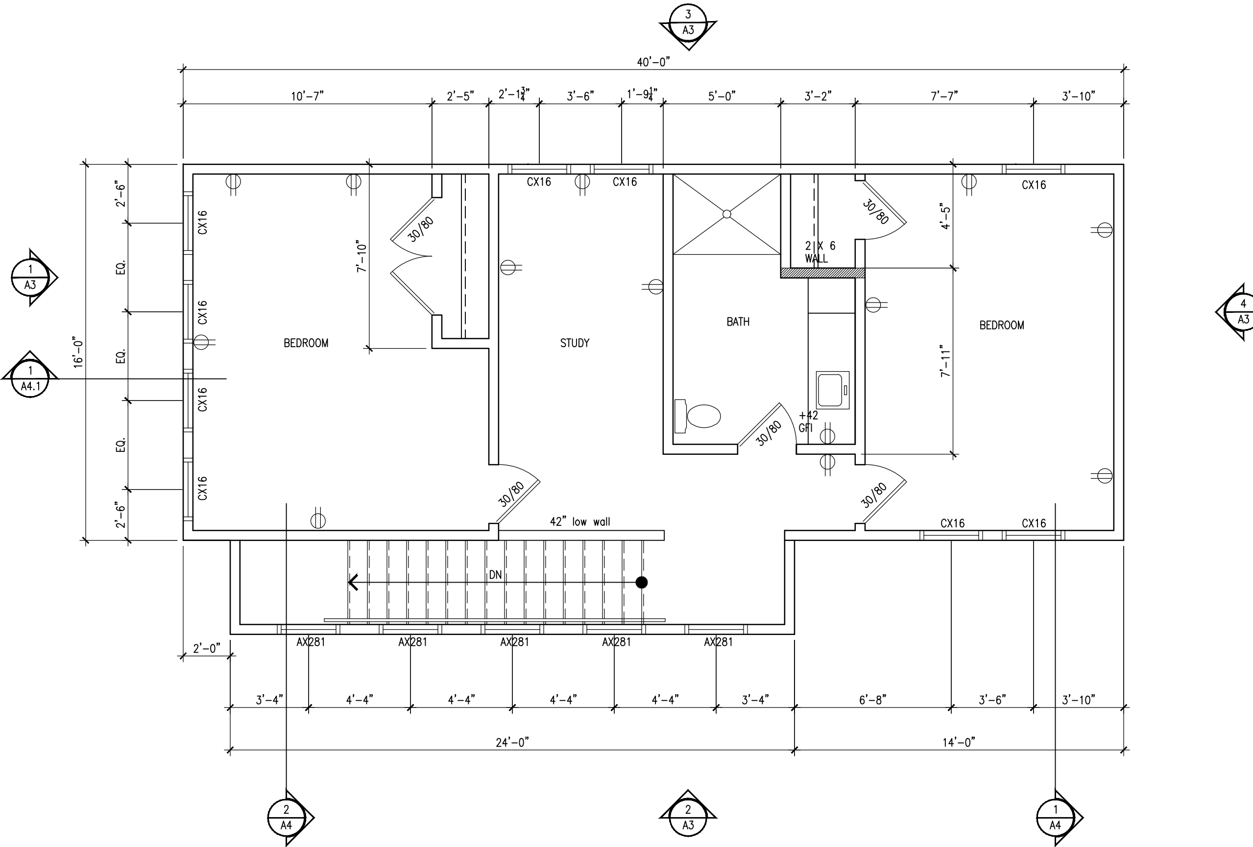
2 SECOND FLOOR SCALE: 1/4"=1'-0"
