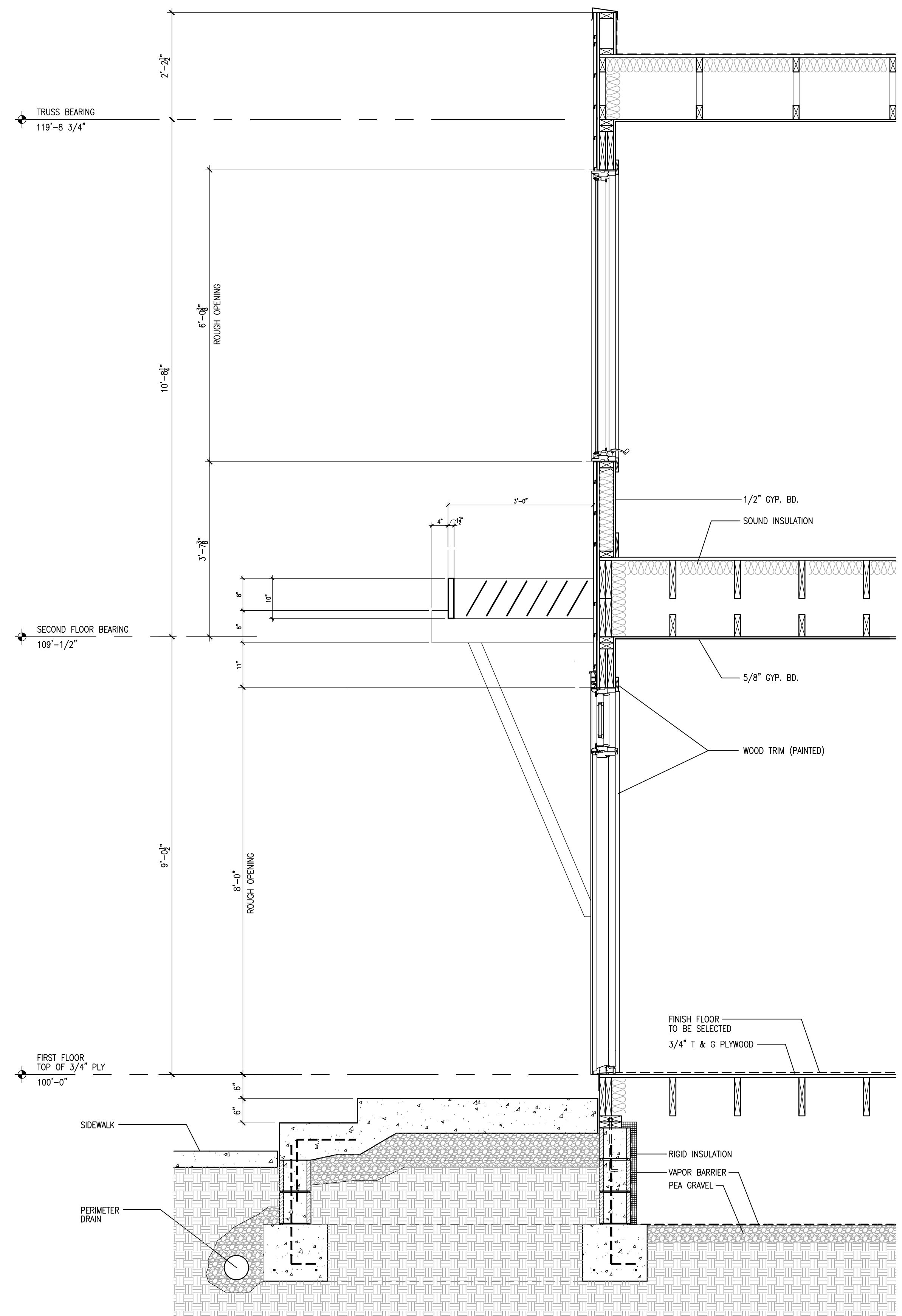
① BUILDING SECTION SCALE: 3/4"=1'-0"
