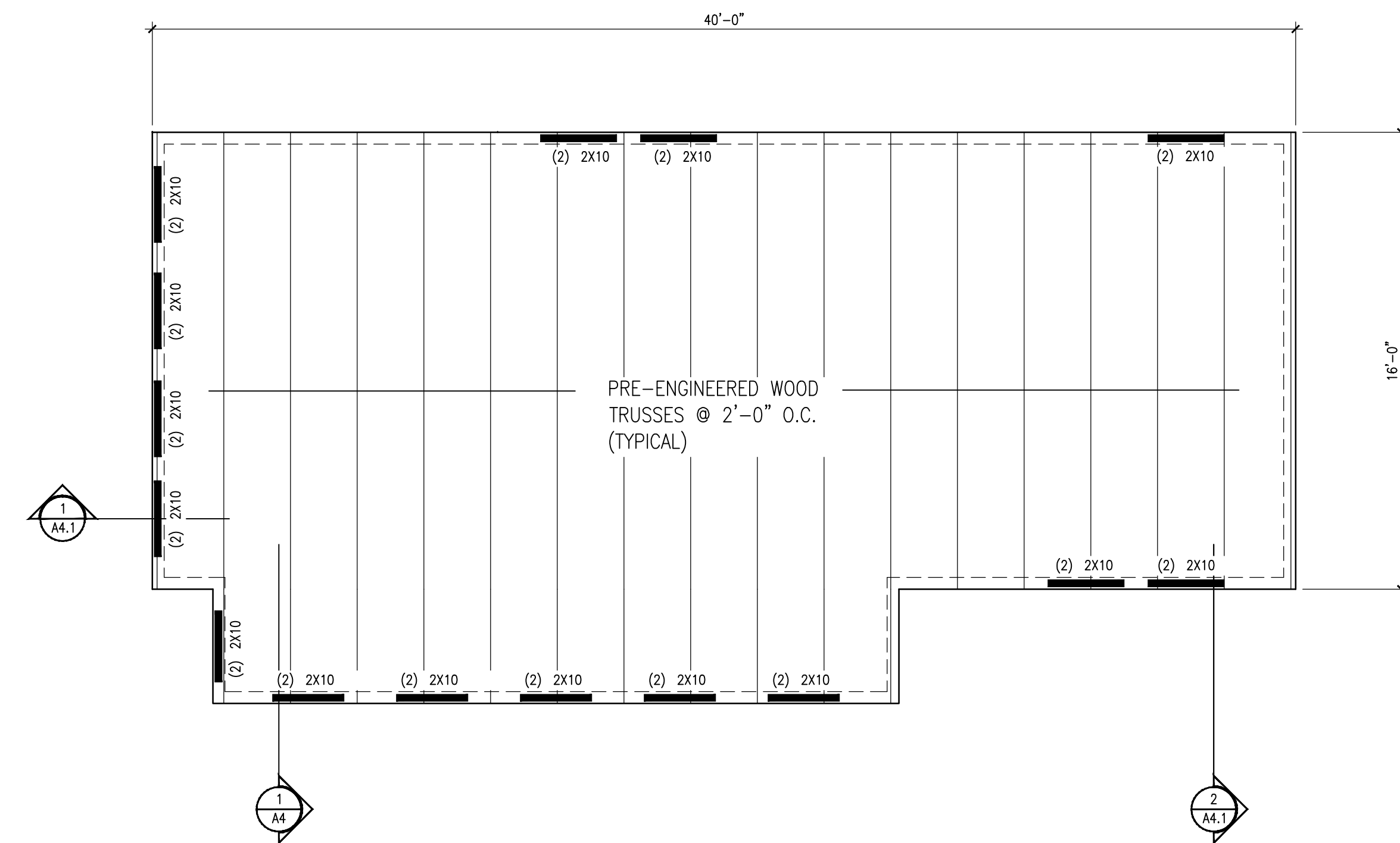
4 ROOF FRAMING PLAN SCALE: 1/4"=1'-0"
