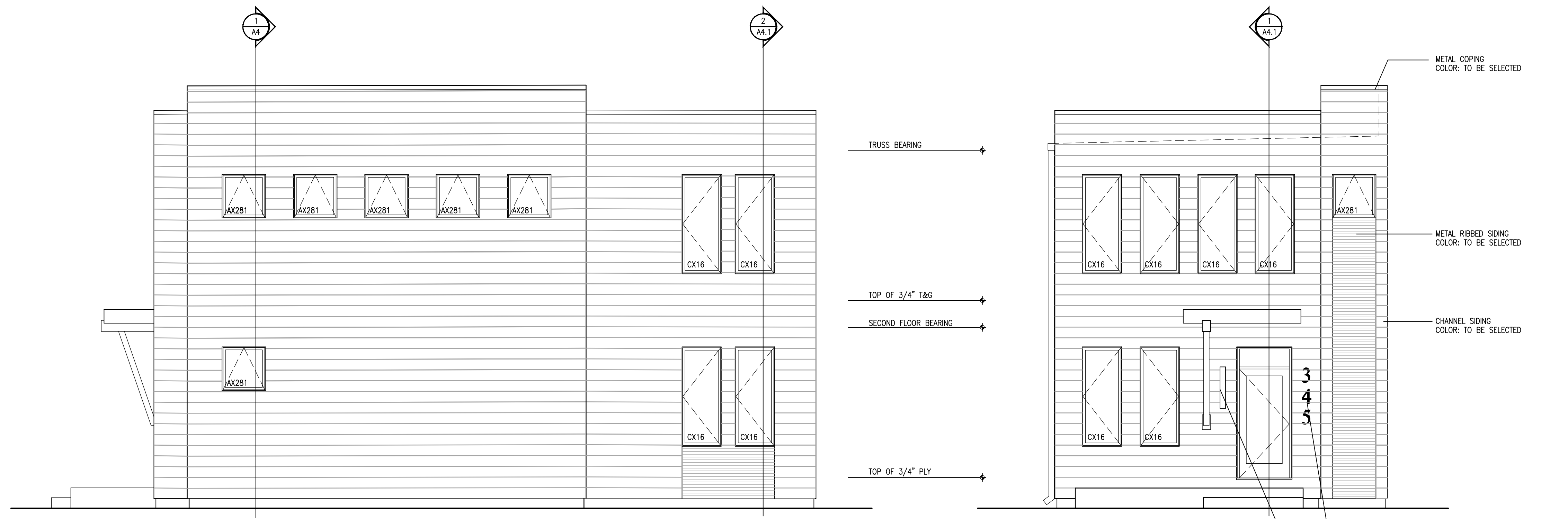
② SIDE ELEVATION SCALE: 1/4"=1'-0"
